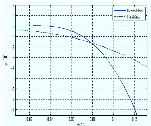
Figure 15. Amplitude characteristic of overall filter – Pass-band
