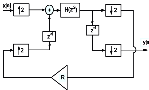
Figure 6. A cascade of two identical filters realized by using a single filter
