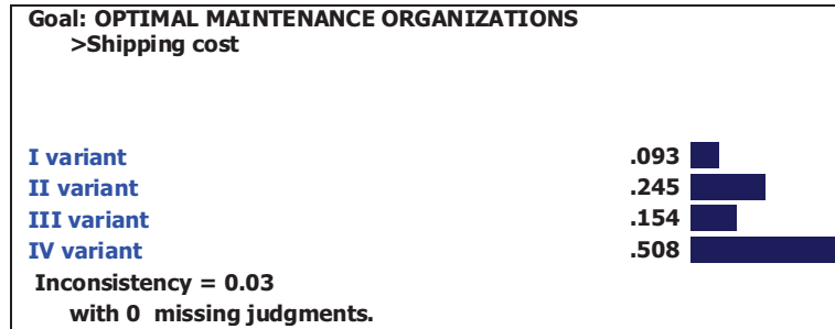
Fig. 6 – The importance of of alternatives against the criteria K4 (transport costs due to maintenance of the devices).
